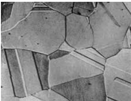
Photomicrograph of austenite
