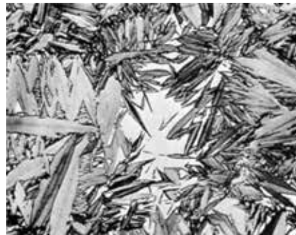
Photomicrograph of martensite
