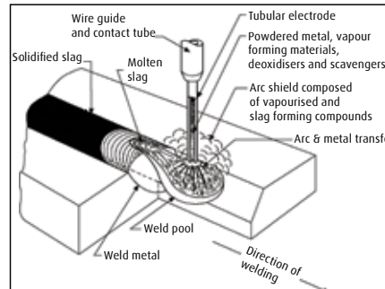
Open Arc Flux Cored Arc Welding (FCAW)
